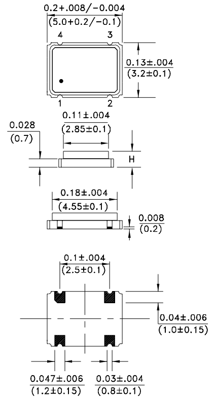
Bottom view Recommended land pattern
