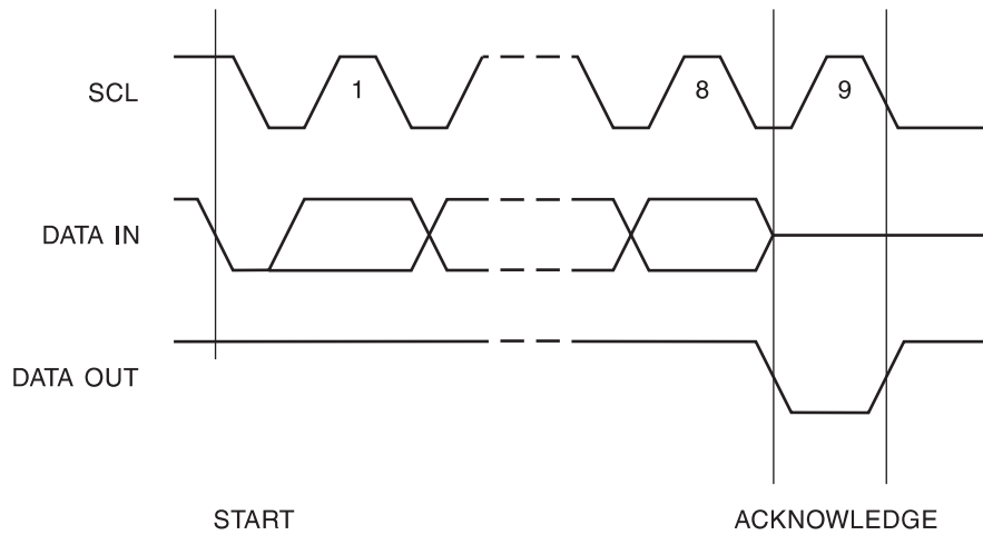
Figure 6. Output Acknowledge
