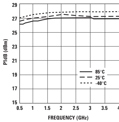
Figure 21. P1dB vs. Temp and Freq tuned for optimal OIP3 at 4.5V, 200 mA.
