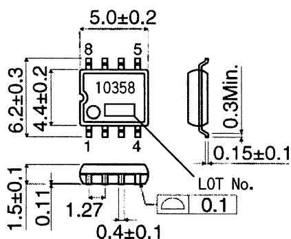
BA10358F(SOP8) (Unit:[mm])
