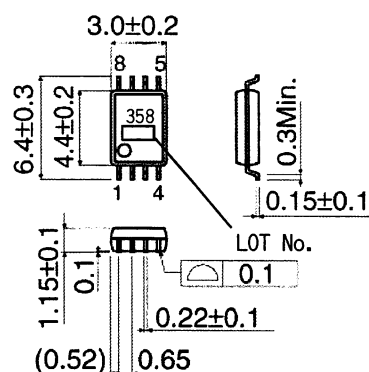
BA10358FV(SSOP-B8) (Unit:[mm])
