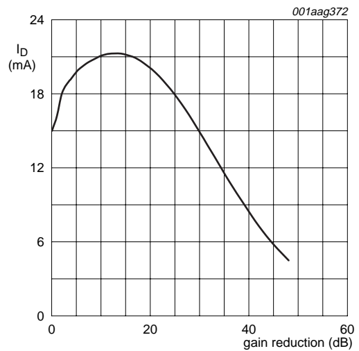
V_{DS(B)} = 5 \text{ V} ; V_{GG} = 5 \text{ V} ; V_{DS(A)} = V_{G1-S(A)} = 0 \text{ V} ; R_{G1} = 86 \text{ k}\Omega (connected to V_{GG} ); f = 50 \text{ MHz} ; T_{amb} = 25 \text{ }^\circ\text{C} ; see Figure 34 .
