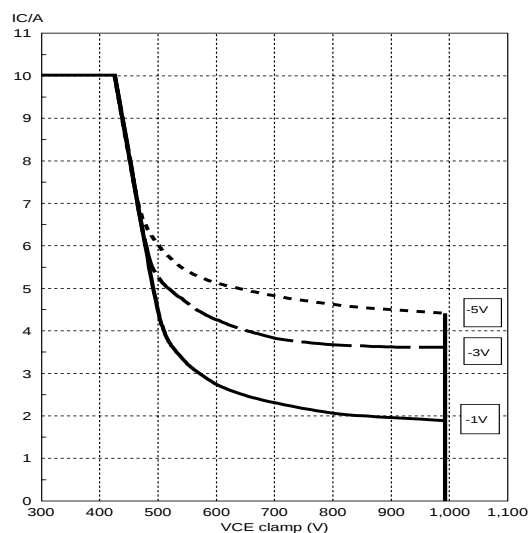
Fig.13. Reverse bias safe operating area ( T_j < T_{jmax} ) for -V_{be} = 5V, 3V & 1V
