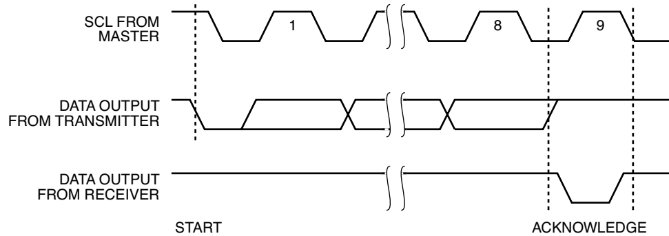
Figure 3. Acknowledge Timing
