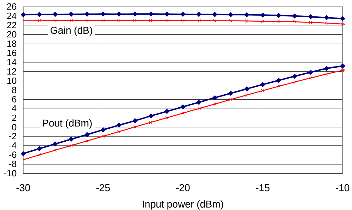
Gain &amp; Output power @ 28–30 GHz
