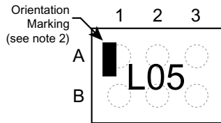
TOP VIEW (Bumps Down View)
