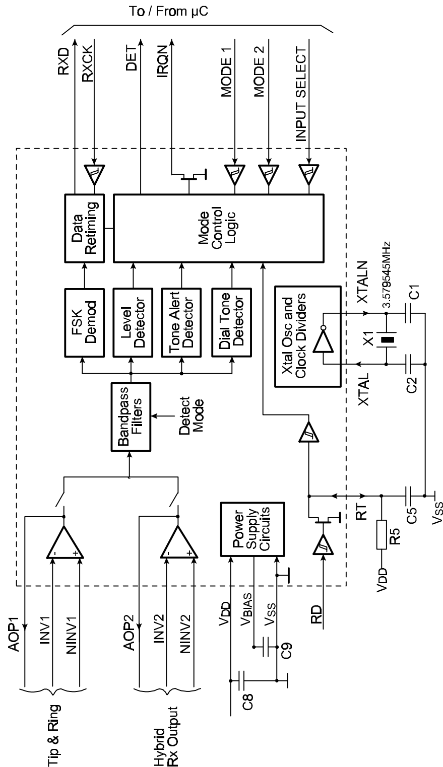
Figure 1 : Block Diagram
