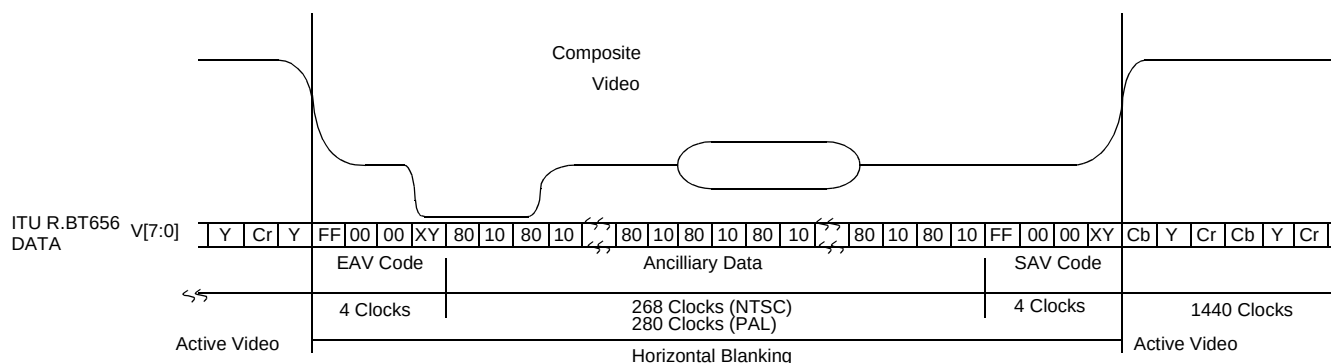
Figure 11. CCIR656 Input Mode Timing
