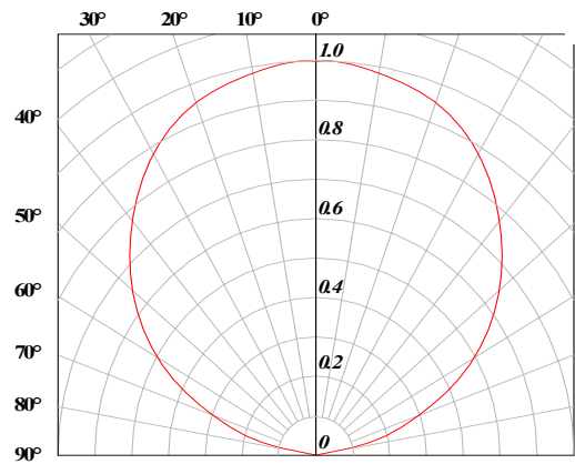
Radiation Pattern
