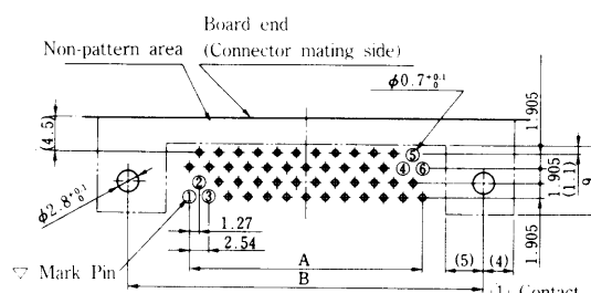
(14, 26, 50 pins)
