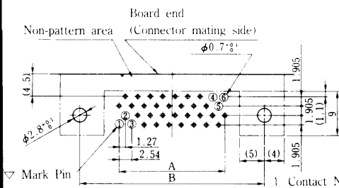
(20, 36, 68 pins)
