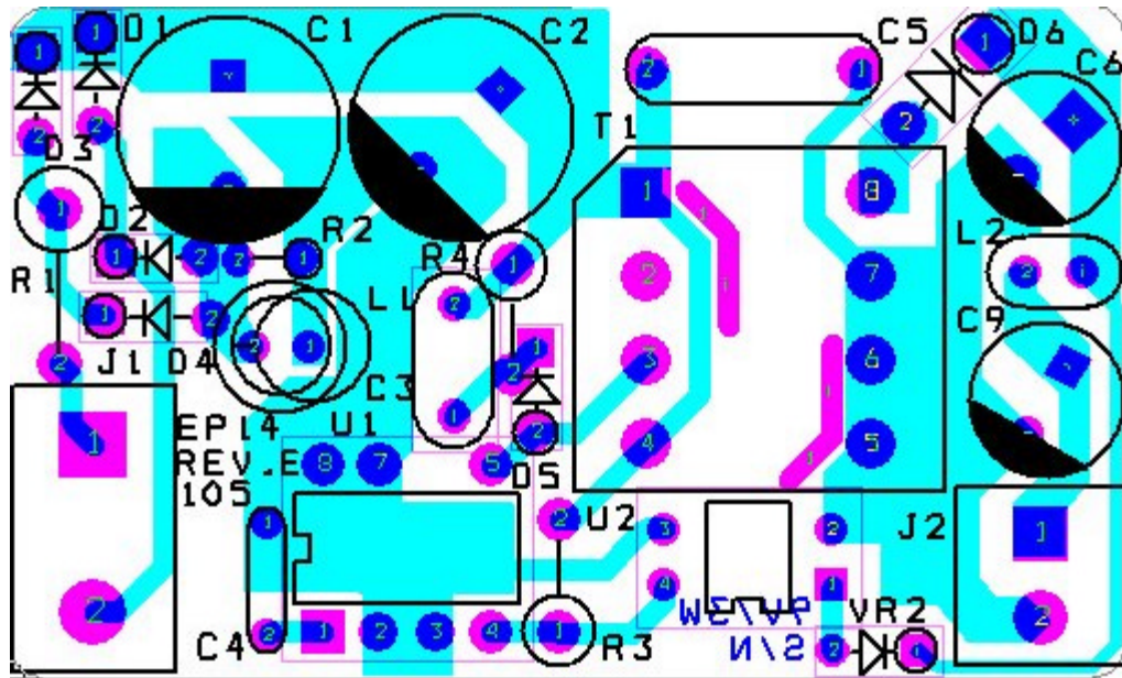
Figure 3. PCB Layout (2.0 × 1.2 × 0.75")
