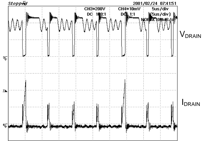
Figure 22. V DRAIN & I DRAIN (200 V & 0.1 A/div) at 3 W Load, 265 V AC Input. (5 µs/div)
