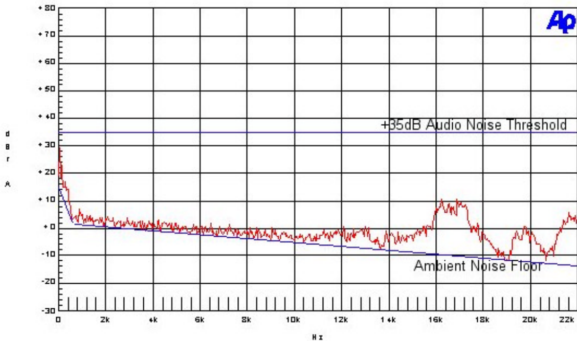
Figure 12. Acoustic Emissions Spectrum, 230 V AC Input, 9 V, 0.21 A Output
