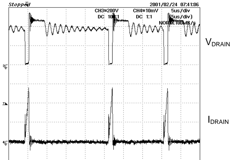
Figure 23. V DRAIN & I DRAIN (200 V & 0.1 A/div) at 3 W Load, 265 V AC Input. (5 µs/div)
