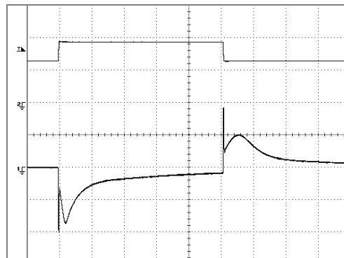
Figure 21 - 230 VAC Transient Response. 75%-100%-75% Load Step. Top: Load Current, 2 A/div. Bottom: Voltage at Supply Output 100 mV, 1 ms/div.
