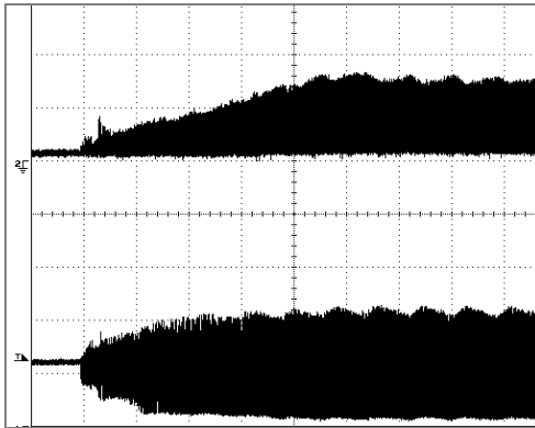
Figure 18 - 90 VAC Input and Maximum Load. Upper: I_{\text{DRAIN}} , 0.5 A/div. Lower: V_{\text{DRAIN}} , 100 V, 10 ms/div.
