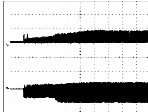
Figure 19 - 265 VAC Input and Maximum Load. Upper: I_{\text{DRAIN}} , 0.5 A/div. Lower: V_{\text{DRAIN}} , 200 V, 10 ms/div.
