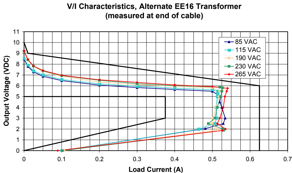
Figure 31 – Line and Load Regulation, Alternative EE16 Transformer Design.
