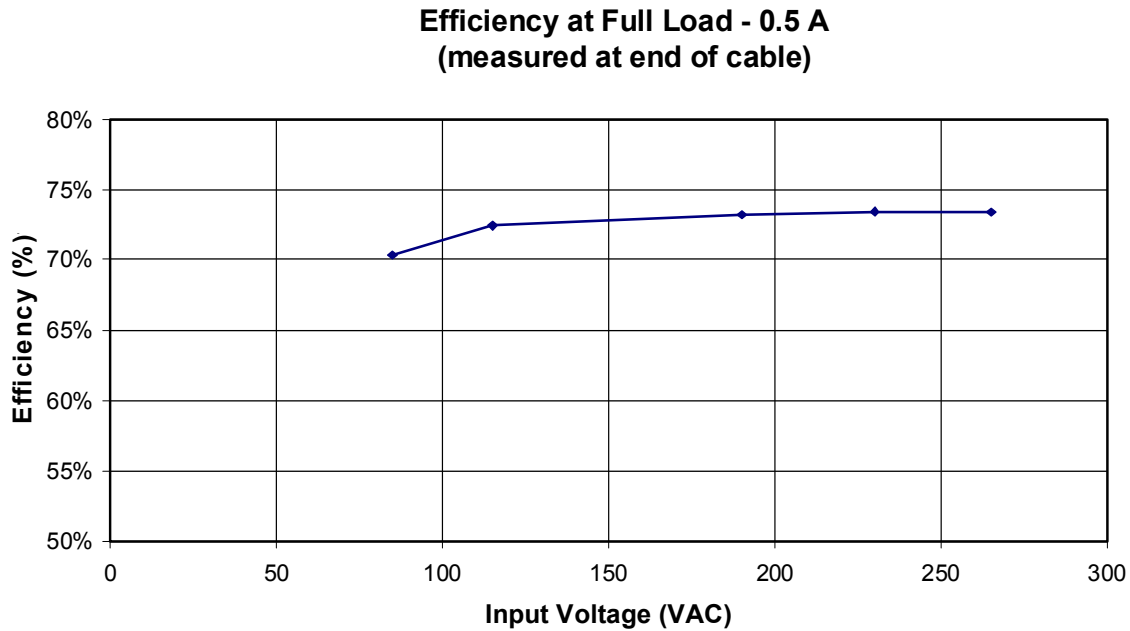
Figure 29 – Efficiency vs. Input Voltage, Alternate EE16, Full Load, Room Temperature, 60Hz.
