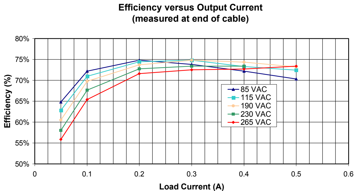
Figure 30 – Efficiency vs. Output Load, Alternate EE16, Room Temperature, 60Hz.
