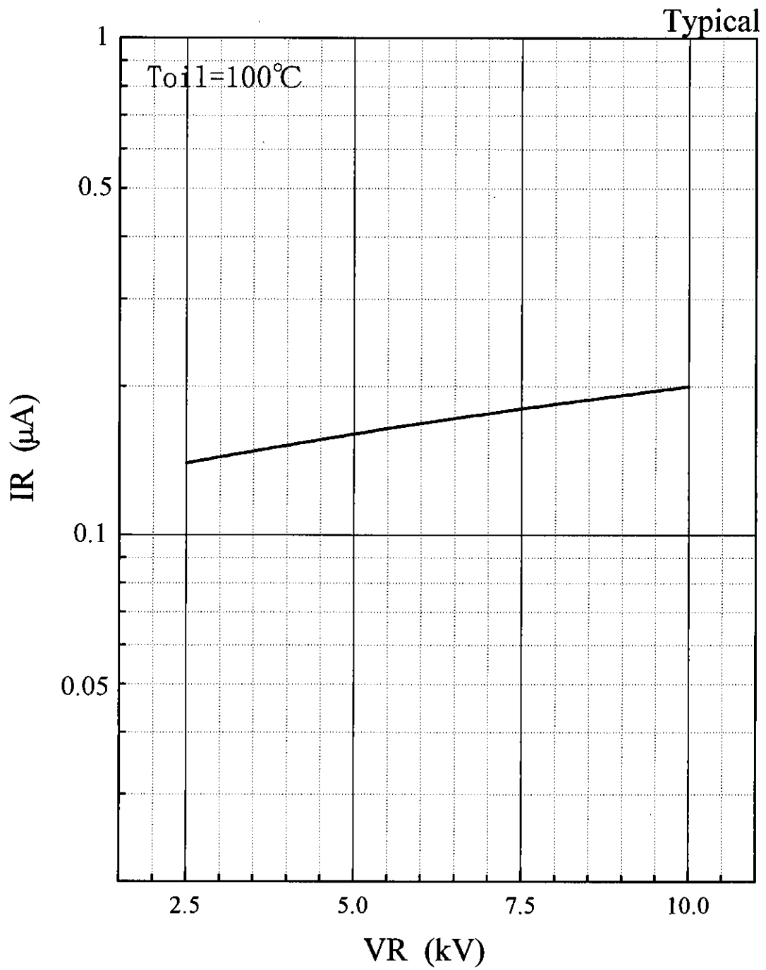
Fig.2 Reverse characteristic[VR-IR]
