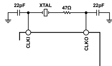
Figure 47. Crystal Connection
