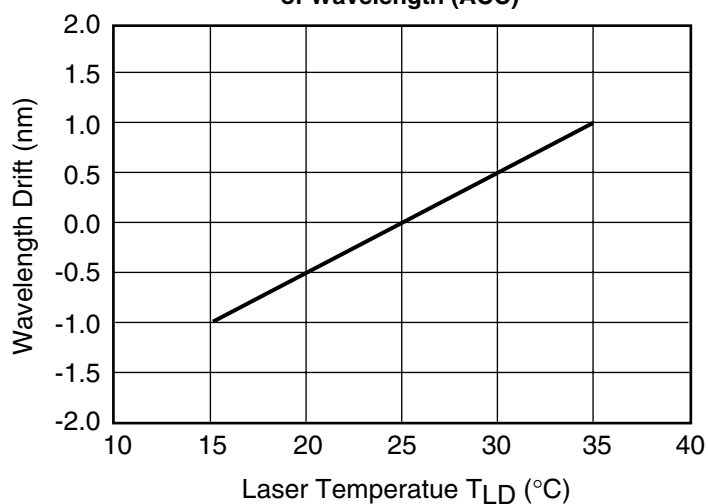
Fig. 2 Laser Temperature Dependence of Wavelength (ACC)
