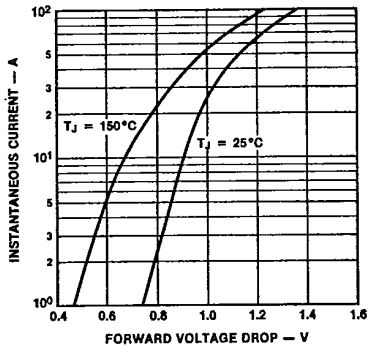
Figure 1 Maximum Forward Voltage Drop
