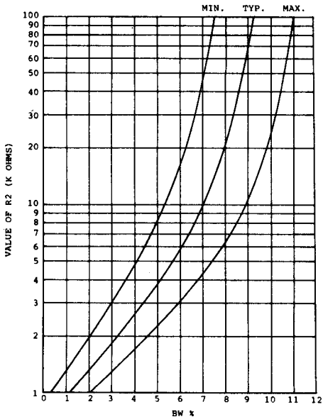
GRAPH 6 GRAPH SHOWING VALUE OF R2 (KΩ) TO YIELD SELECTED BANDWIDTH (%)
