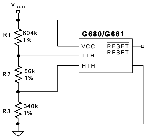
Figure 2. Example Circuit
