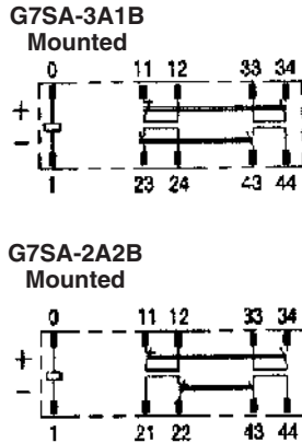
Terminal Arrangement/Internal Connection Diagram (Bottom View)
