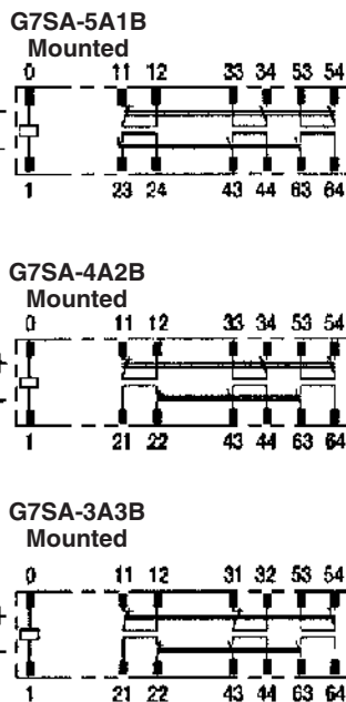
Terminal Arrangement/Internal Connection Diagram (Bottom View)
