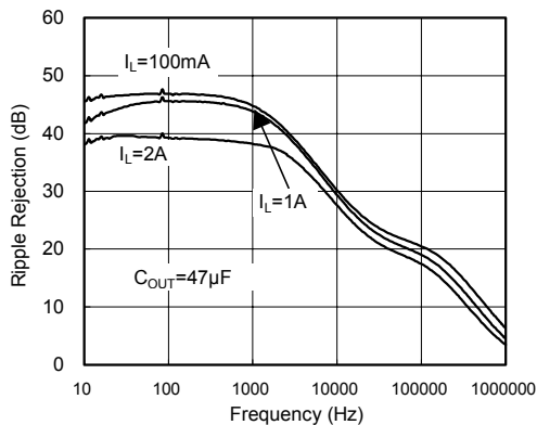
Ripple Rejection
