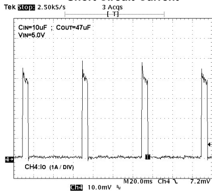
Short Circuit-Current
