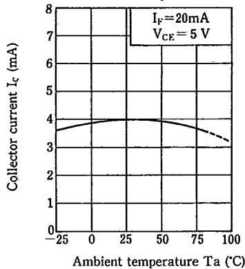
Fig. 7 Collector Current vs. Ambient Temperature
