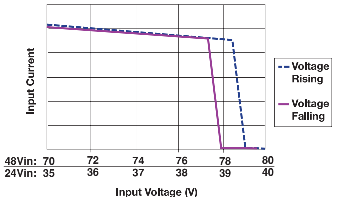
Overvoltage Lockout
