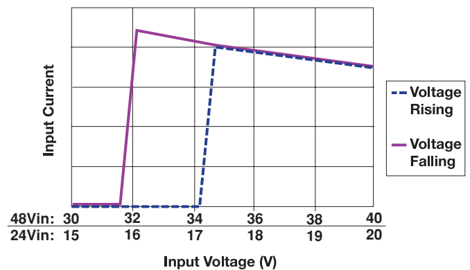
Undervoltage Lockout
