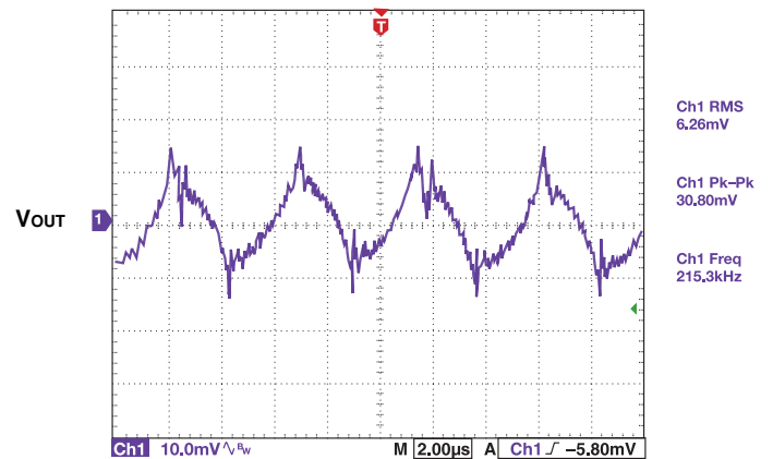
Voltage Ripple
