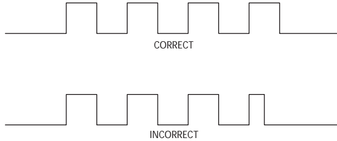
Figure 3-4: Burst Clock
