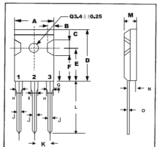
TO-247 (3P)
