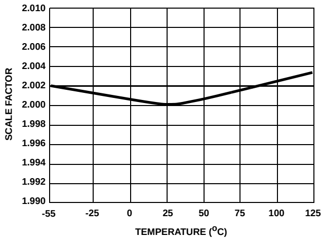
FIGURE 31. SCALE FACTOR vs TEMPERATURE
