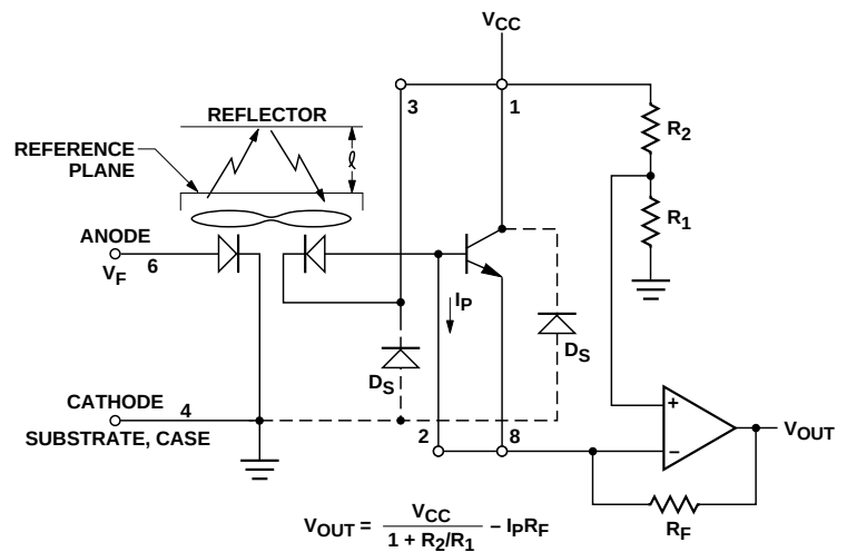
Figure 15. Photodiode Interconnection.
