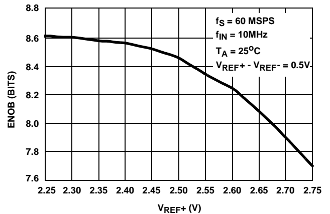
FIGURE 8. EFFECTIVE NUMBER OF BITS (ENOB) vs V REF+
