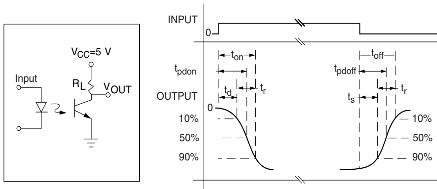
Figure 11. Switching Test Circuit
