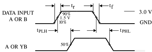
Figure 1. Switching Waveforms
