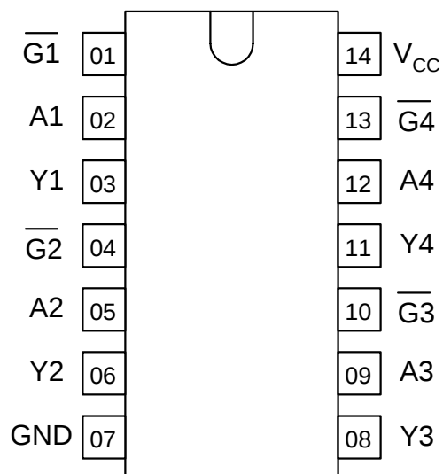
Pinout
