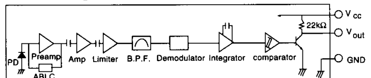
Block Diagram:
