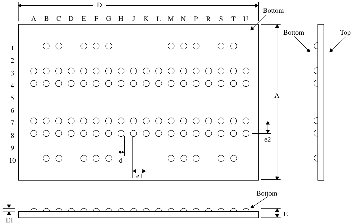
Figure 4: Center-Bonded WBGA Package
