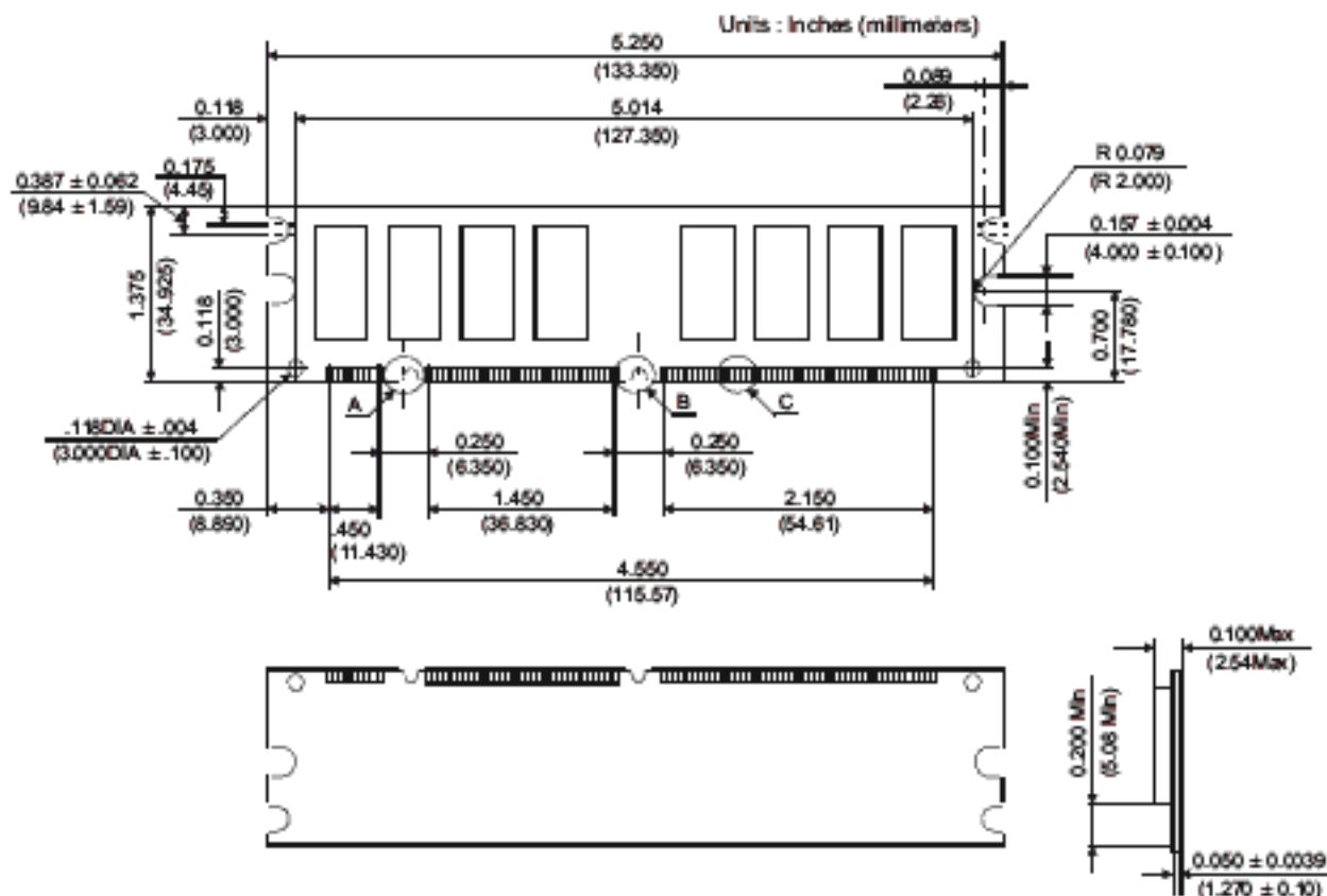
Figure 1: KVR100X64C2/64 168-Pin SDRAM Module
