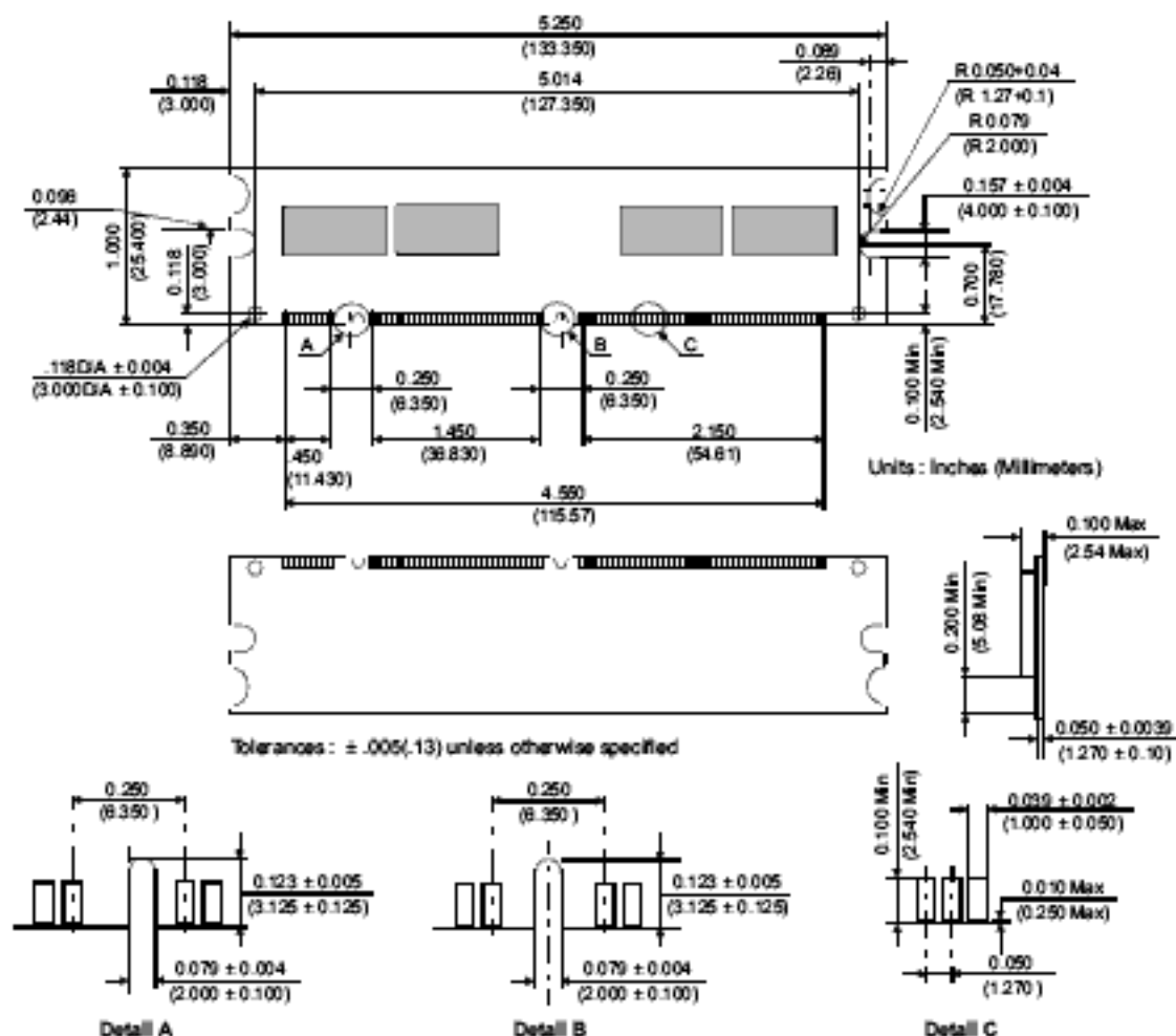
Figure 1: KVR133X64C3L/128 168-Pin SDRAM Module
