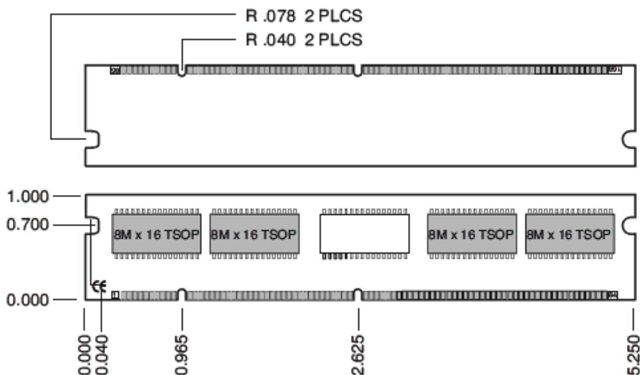
Figure 1: KVR133X64C3L/64 168-Pin SDRAM Module
