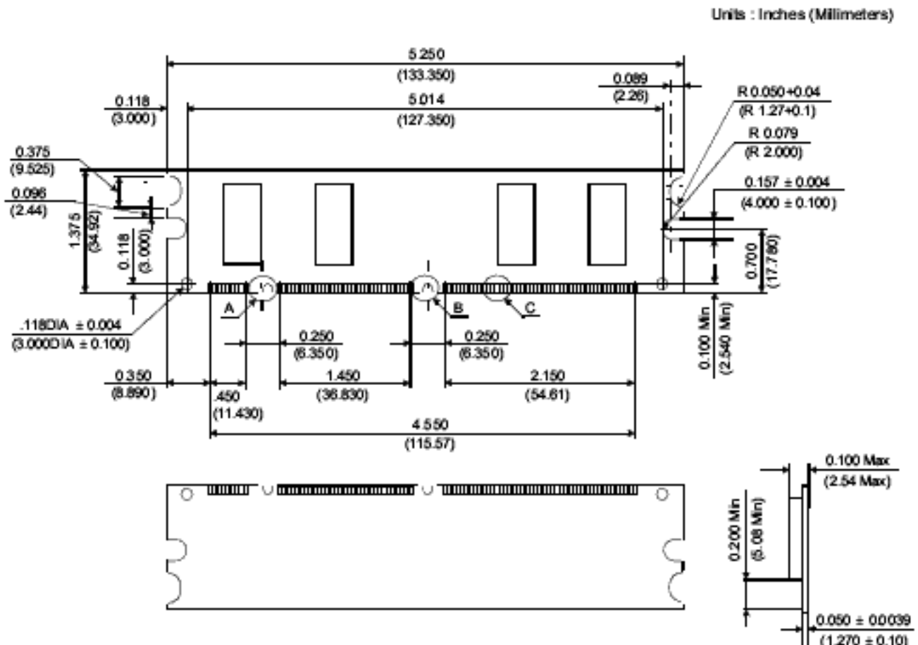
Figure 1: KVR133X64C3SS/128 168-Pin SDRAM Module
