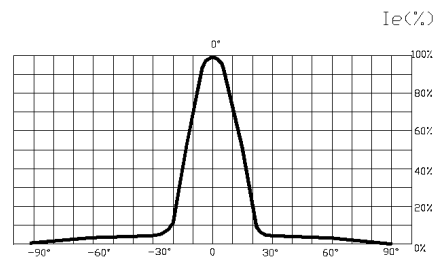
FIG.6 FAR FIELD PATTERN
