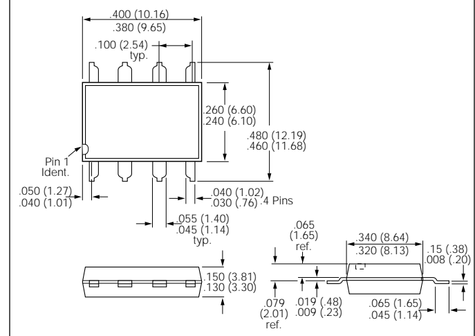
"S" Bend Leads: Package Dimensions in Inches (mm)
