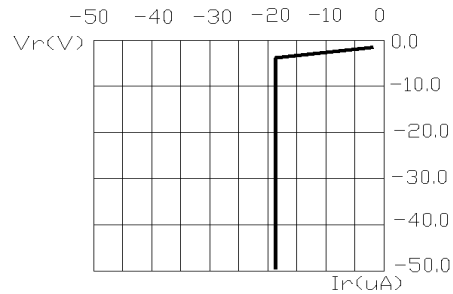
FIG.2 REVERSE CURRENT VS. REVERSE VOLTAGE.
