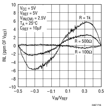
Figure 16. INL vs Differential Input Voltage and Reference Source Resistance for C_{REF} > 1\mu\text{F}
