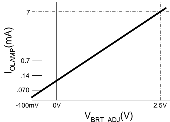
Figure 9 – Average Lamp Current vs. V_{\text{BRITE}} Voltage (per Lamp)
