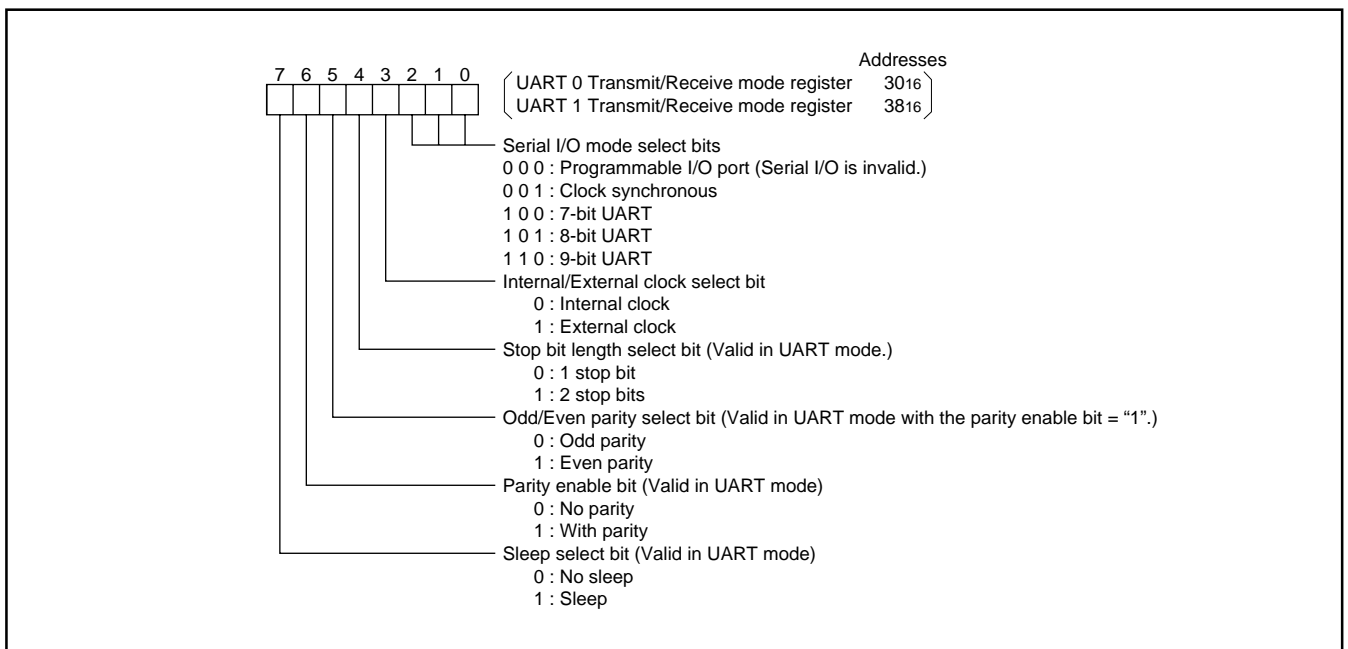
Fig. 51 Bit configuration of UARTi transmit/receive mode register
