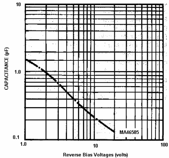
CAPACITANCE vs. VOLTAGE GAMMA = 1.00 +/-10% FROM 2-12V0lts
