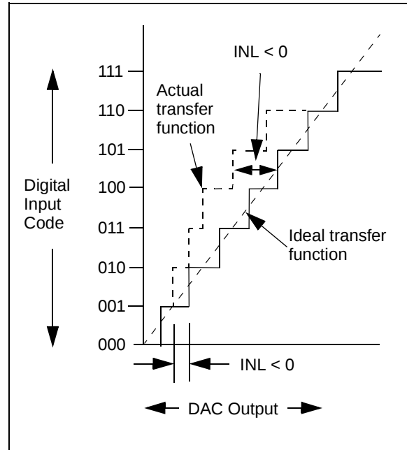
FIGURE 4-1: INL Accuracy.
