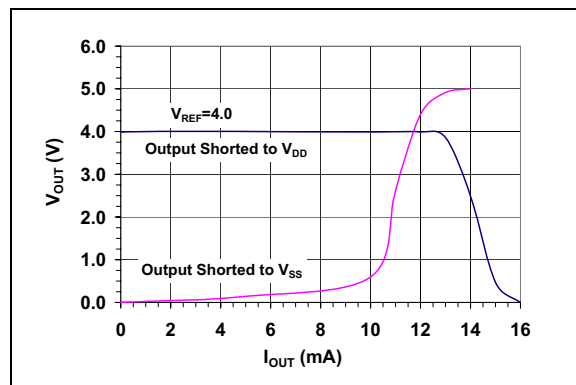
FIGURE 2-28: I_{OUT} vs V_{OUT} . \text{Gain} = 1 .
