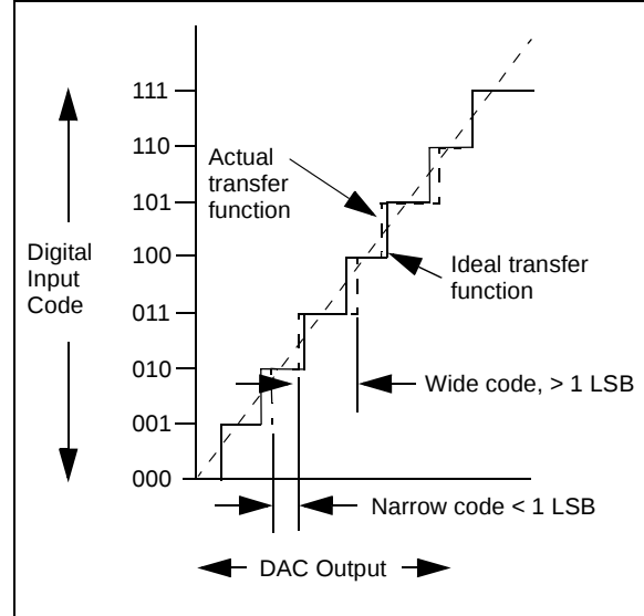
FIGURE 4-2: DNL Accuracy.
