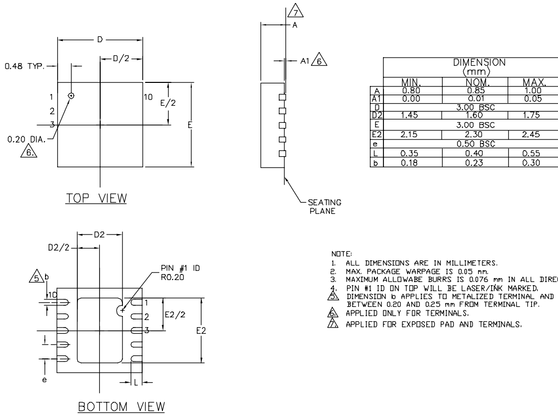
10-Pin 3mm x 3mm MLF™ (ML)
