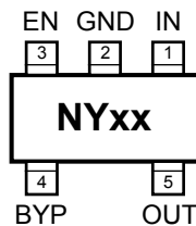
MIC5259-x.xBD5 ThinSOT™-23-5 (D5) (Top View)
